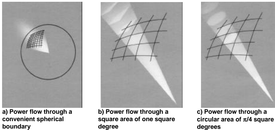
Figure 3. Simplified assumptions as to the shape of the radiated power yield approximate calculations of directive gain.
