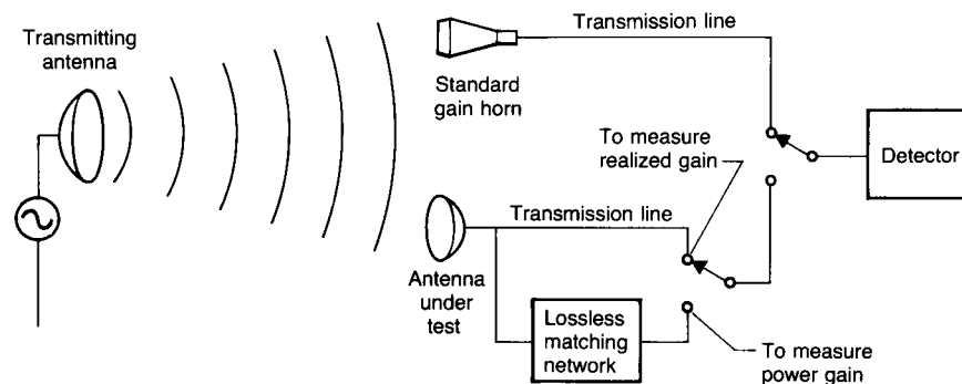
Figure 6. Power gain and realized gain measurements.
