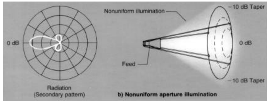
Figure 5. Field distributions, and radiation patterns produced, when a parabolic reflector's aperture is uniformly and nonuniformly illuminated.
