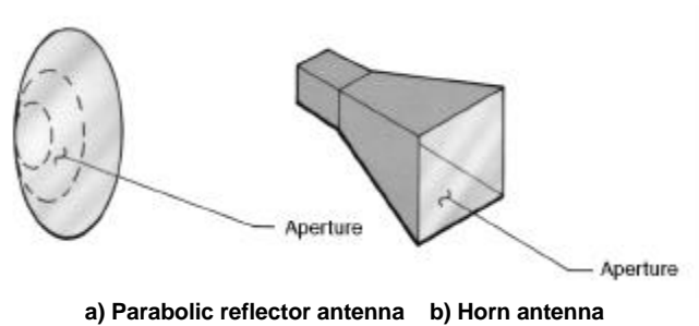
a) Parabolic reflector antenna b) Horn antenna Figure 4. Physical apertures of parabolic reflector- and horn-type antennas.
